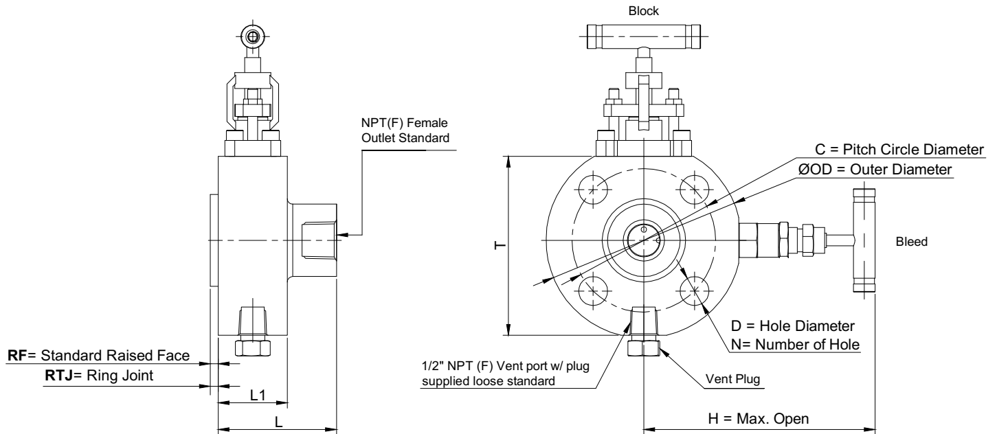
OS&Y Bonnet Dimensions (inches)
