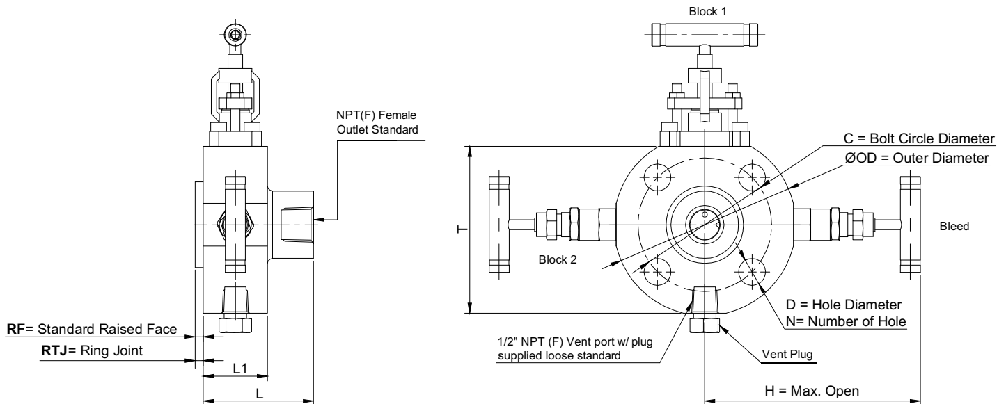
OS&Y Bonnet Dimensions (inches)
