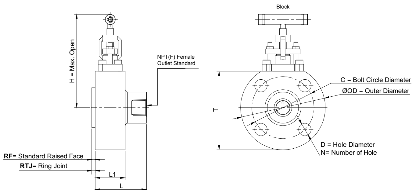
OS&Y Bonnet Dimensions (inches)
