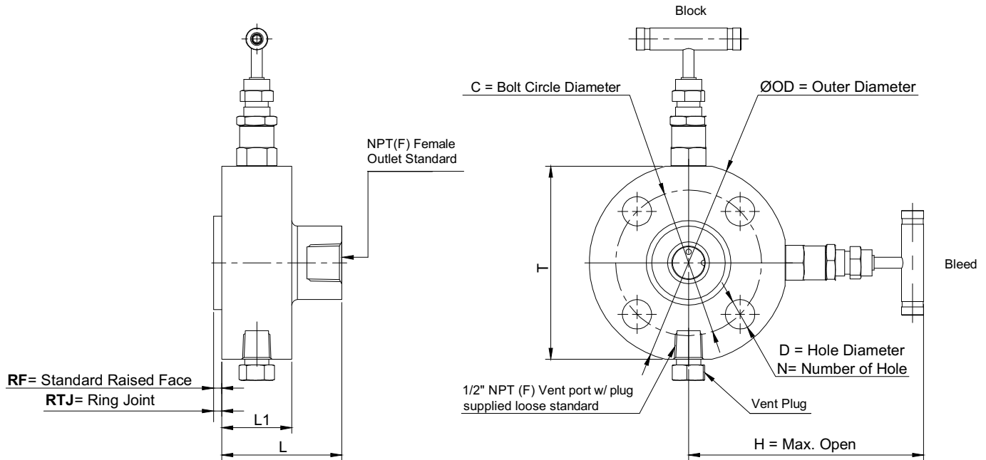
Standard Screwed Bonnet Dimensions (inches)
