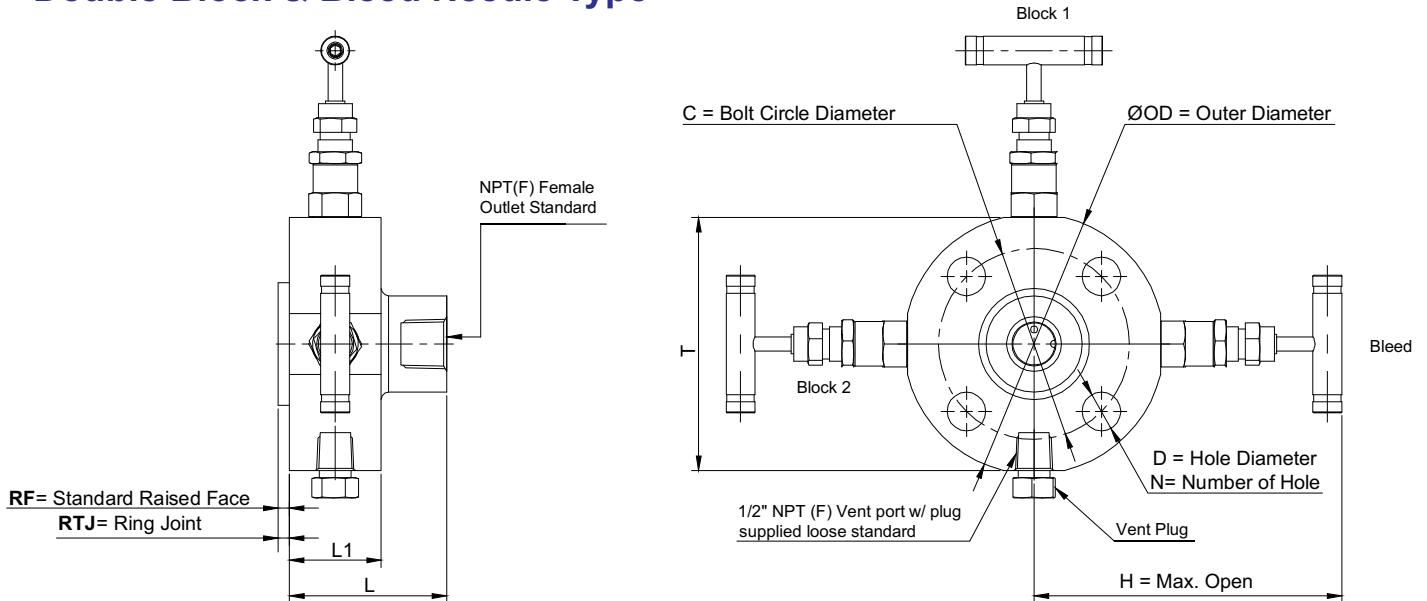
Standard Screwed Bonnet Dimensions (inches)
